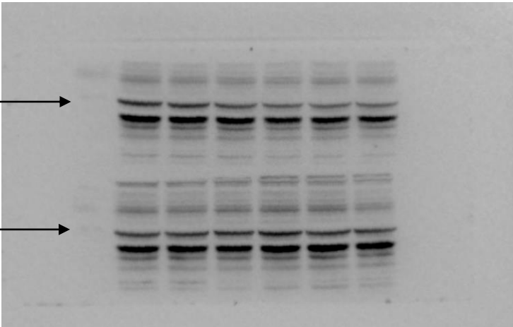
Figure 3A, MEL-1A/B—43KD
