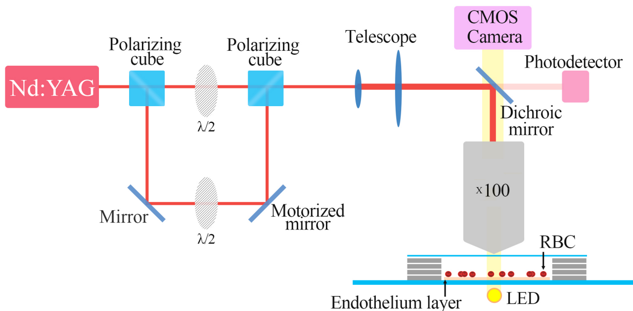
Fig. 1. Schematic representation of dual-channel optical tweezers. A Nd:YAG laser beam is divided into two beams of approximately equal intensity and opposite polarization by a polarizing cube. One beam passes through an additional polarizing cube unchanged and forms the stationary optical trap. The other beam travels through a mirror system that allows independent positional adjustment and creates a movable optical trap. Half-wave plates regulate the laser intensity, controlling the trapping force. A telescope expands the beam to create optimal conditions for trapping red blood cells (RBCs). A dichroic mirror transmits a small fraction of the laser light to a photodetector for real-time intensity measurement. Most of the light is reflected into the objective, which creates the optical traps. A cuvette is positioned beneath the objective and consists of a slide, a monolayer of human umbilical vein endothelial cells (HUVECs), an RBC suspension in autologous plasma at low hematocrit, and a coverslip. LED illumination and a CMOS camera were used to enable sample visualization. LED, light-emitting diode; CMOS, complementary metal-oxide-semiconductor.
