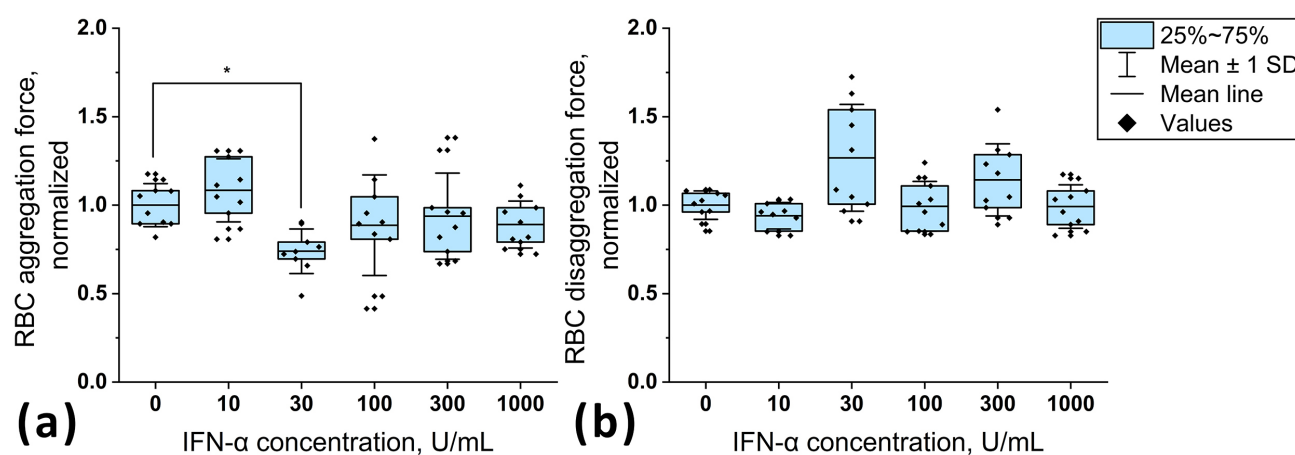
Fig. 5. Normalized aggregation and disaggregation forces of RBCs in the presence of long-term IFN- \alpha -treated HUVECs. (a) Normalized RBC aggregation forces in the presence of HUVECs. The box indicates the Q1–Q3 interval; the horizontal line indicates the mean; whiskers indicate the mean \pm 1 standard deviation (SD); points indicate individual values. HUVECs were incubated with the indicated concentration of IFN- \alpha for 24 hours. IFN- \alpha was not added to blood plasma containing RBCs. Statistical analyses were performed using the Mann–Whitney U test. The asterisk indicates statistical significance of the difference between samples (* p < 0.05 ). Each point corresponds to one measurement. (b) Normalized RBC disaggregation forces in the presence of HUVECs. The box indicates the Q1–Q3 interval; the horizontal line indicates the mean; whiskers indicate the mean \pm 1 standard deviation (SD); points indicate individual values. HUVECs were incubated with the indicated concentration of IFN- \alpha for 24 hours. IFN- \alpha was not added to blood plasma containing RBCs. Statistical analyses were performed using the Mann–Whitney U test. The asterisk indicates statistical significance of the difference between samples (* p < 0.05 ). Each point corresponds to one measurement.
