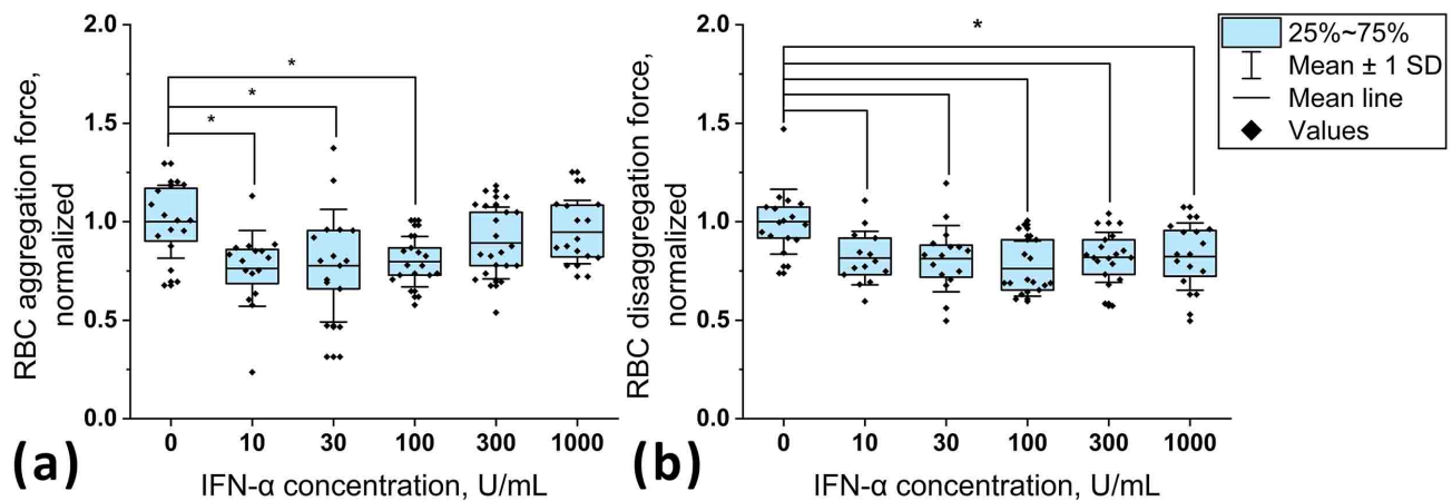
Fig. 3. Normalized aggregation and disaggregation forces of RBCs in the presence of short-term IFN- \alpha -treated HUVECs. (a) Normalized RBC aggregation forces in the presence of HUVECs. The box indicates the Q1–Q3 interval, the horizontal line indicates the mean, whiskers indicate the mean \pm 1 standard deviation (SD), and points indicate individual values. IFN- \alpha was added to blood plasma containing RBCs in the cuvettes before measurements. Statistical analyses were performed using the Mann–Whitney U test. The asterisk indicates statistical significance of the difference between samples ( *p < 0.05 ). Each point corresponds to one measurement. (b) Normalized RBC disaggregation forces in the presence of HUVECs. The box indicates the Q1–Q3 interval, the horizontal line indicates the mean, whiskers indicate the mean \pm 1 standard deviation (SD), and points indicate individual values. IFN- \alpha was added to blood plasma containing RBCs in the cuvettes before measurements. Statistical analyses were performed using the Mann–Whitney U test. The asterisk indicates statistical significance of the difference between samples ( *p < 0.05 ). On this graph every sample is statistically significantly lower compared with control values. Each point corresponds to one measurement.
