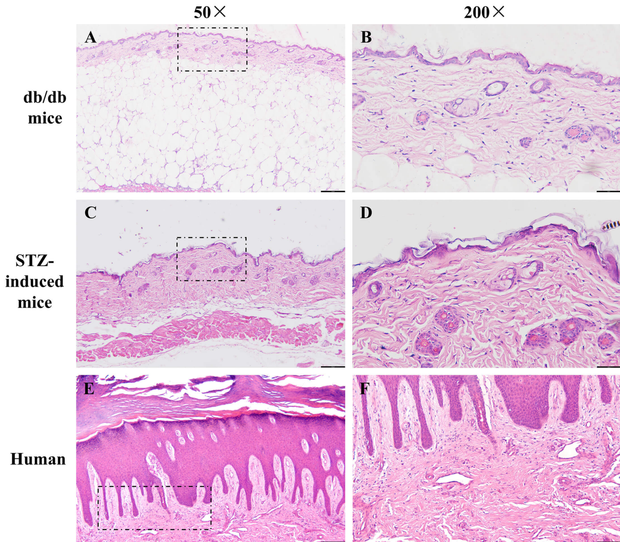
Fig. 1. Histological comparison of skin from db/db mice, STZ mice, and DF patients. Left panels show low-magnification views (50 \times ) of the overall epidermal and dermal architecture, with dashed boxes indicating the regions enlarged in the corresponding right panels (200 \times ). Scale bars: 200 \mu m (50 \times images) and 50 \mu m (200 \times images).
