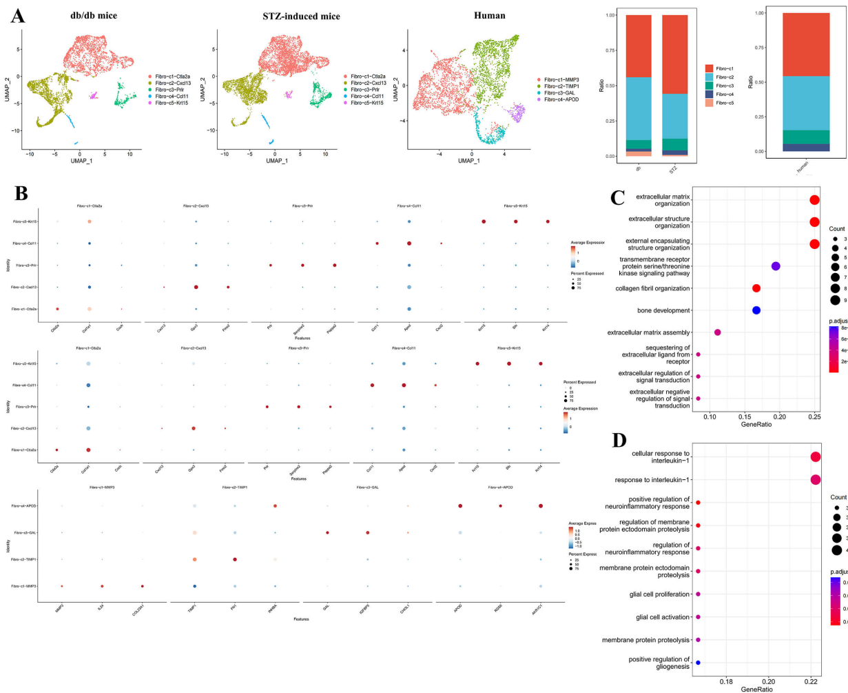
Fig. 5. Fibroblast subclusters and functional enrichment. (A,B) UMAP and the cell proportions of fibroblast subpopulations across groups, and the dot plot of marker gene expression across clusters. (C,D) Functional enrichment analysis of genes from the most abundant fibroblast subpopulation in mice and human skin.
