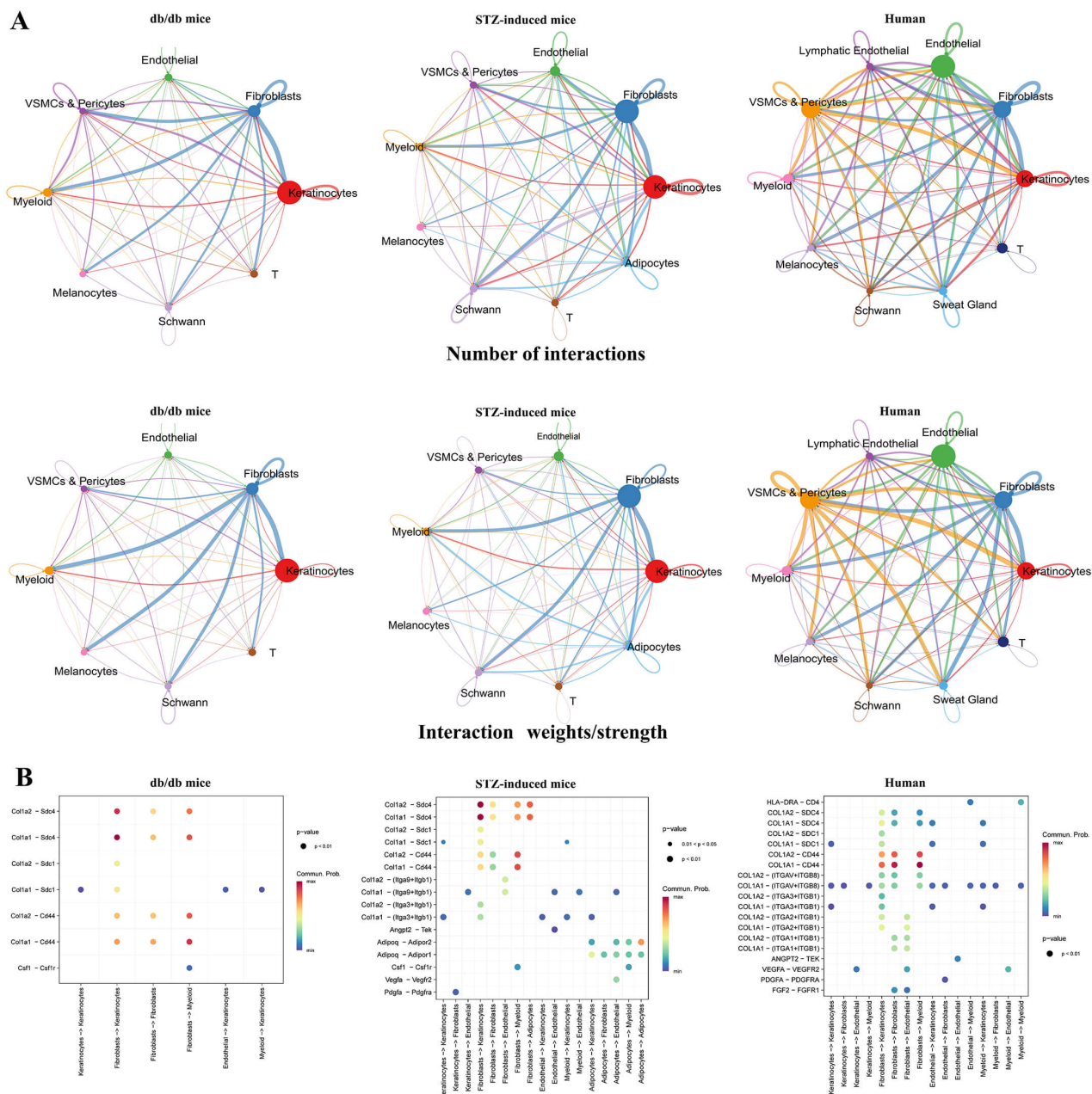
Fig. 3. Cell-cell communication networks. (A) Each node represents a cell population; larger nodes indicate a greater number of cells within that population participating in interactions. Each edge denotes an interaction between the two connected populations; thicker edges indicate stronger interactions, and a greater number of edges connected to a node indicates that the corresponding population engages in more interactions. (B) Ligand-receptor pairs with strong interactions among cell populations.
