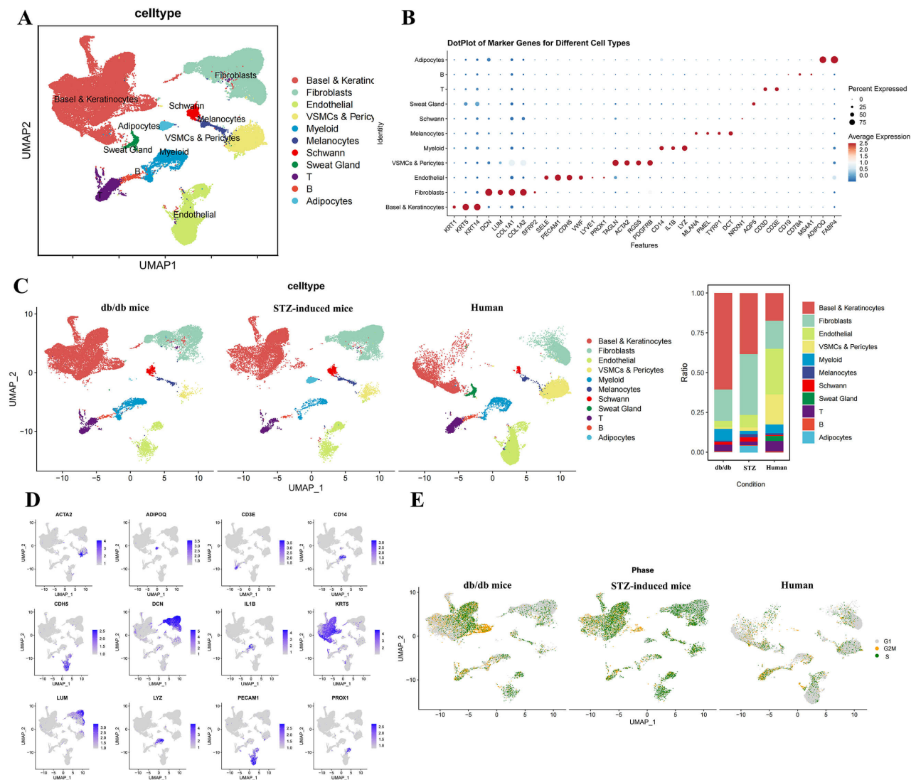
Fig. 2. Overview of single-cell transcriptomes from diabetic mice and human skin. (A) UMAP cell-type distribution shows the clustering results of skin single-cell transcriptomes in UMAP. Each point represents a cell, and the colors correspond to the annotated cell types. (B) The bubble plot shows the expression of representative marker genes across cell types. The bubble size indicates the percentage of cells expressing the gene, and the color of the dots indicates the normalized average expression. (C) UMAP projections, cell-type annotations, and the relative proportions of each cell type are shown separately for the three groups: db/db mice, STZ mice, and human. (D) Marker-subset dimensionality reduction and clustering. (E) In the cell cycle analysis, each dot represents a single cell; different colors denote distinct phases: White indicates the G1 phase, orange indicates the G2 or M phase, and green indicates the S phase. UMAP, Uniform Manifold Approximation and Projection.
