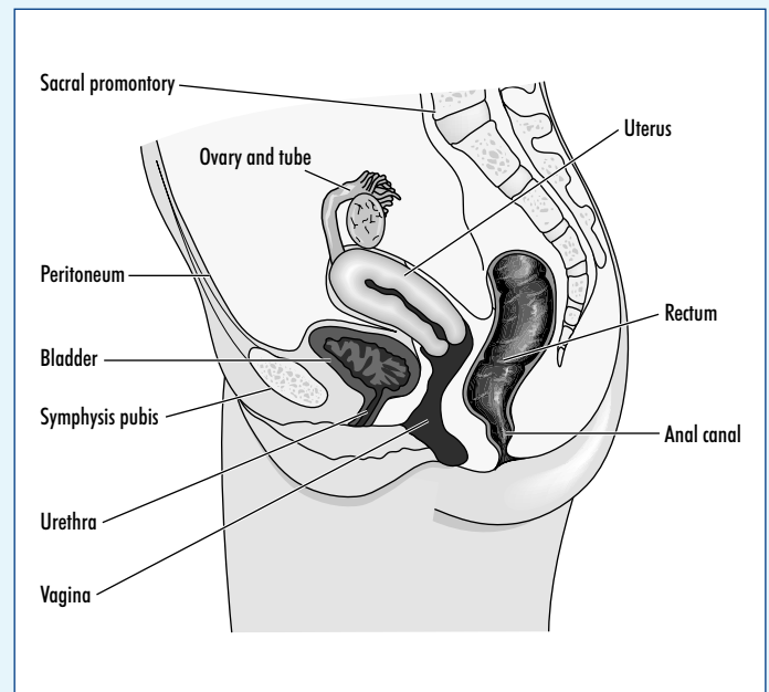
Figure 2. Sagittal section of the female pelvis.
