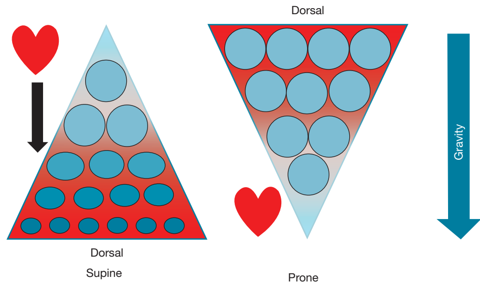
Figure 3. When supine, gravity and the weight of the heart result in compression of dependent dorsal areas of lung and thus hypoventilation. In the prone position, the alveoli become more homogenous and the weight of the heart is instead on the sternum. This leads to increased perfusion of dorsal lung segments with reduced ventilation–perfusion mismatch. Perfusion in the lung remains largely dorsal in both the supine and prone position. Red shading indicates the most perfused lung regions. Adapted from Koulouras et al (2016).
