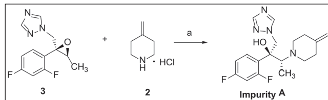
Scheme 2: Formation of Impurity A
