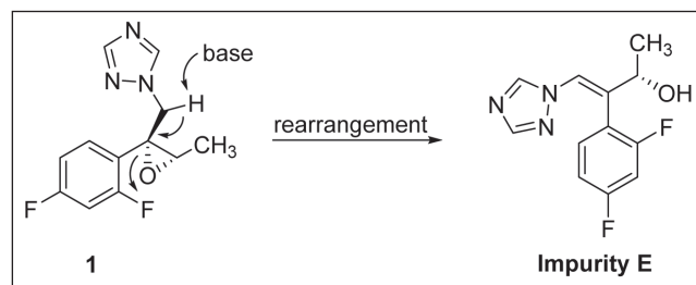
Scheme 6: Formation of Impurity E
