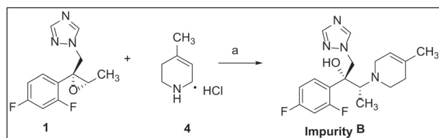
Scheme 3: Formation of Impurity B
