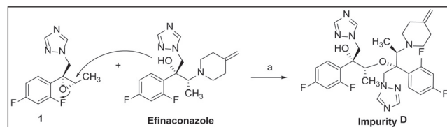
Scheme 5: Formation of Impurity D
