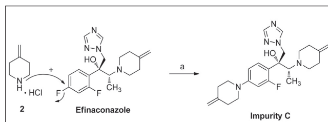
Scheme 4: Formation of Impurity C
