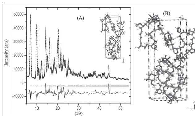
Fig. 3: Diffractogram of SRL adjusted by the Rietveld method (A) and, (B) an SRL unit cell obtained by Rietveld rearrangement.
