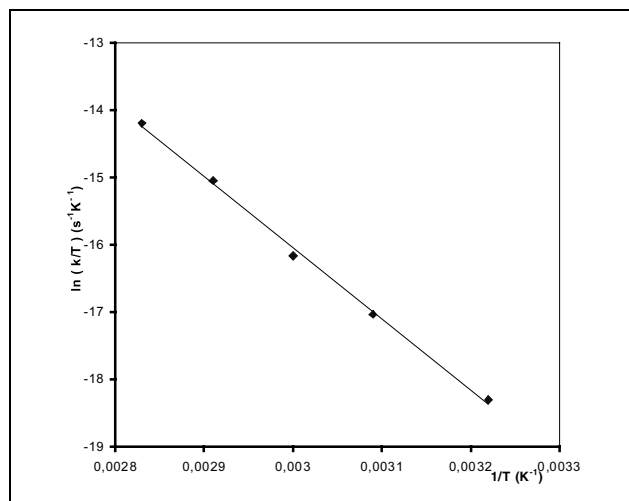
Fig. 3: The \ln k/T vs. 1/T plot of alkaline hydrolysis of cladribine. Enthalpy 88.17 kJ/mol and entropy -66.55 \text{ J/K} \cdot \text{mol}
