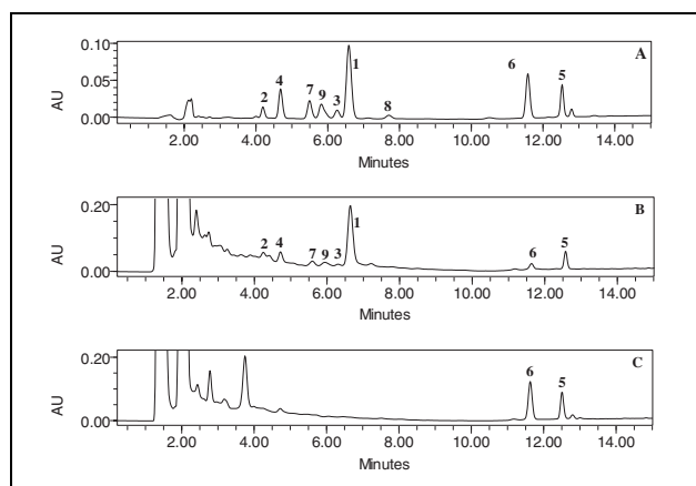
Fig.: A typical HPLC chromatogram of pure neo -clerodane diterpenoidal standards (1–9) (A), and plant extracts (B, C) at 220 nm
