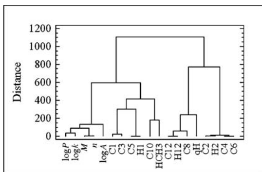
Fig. 2: Cluster analysis of 18 variables (molecule properties) for 62 investigated compounds and surface anaesthetical activity expressed by log A. Ward's clustering method and the Squared Euclidean distance was used. Software Statgraphics Plus 5.1
