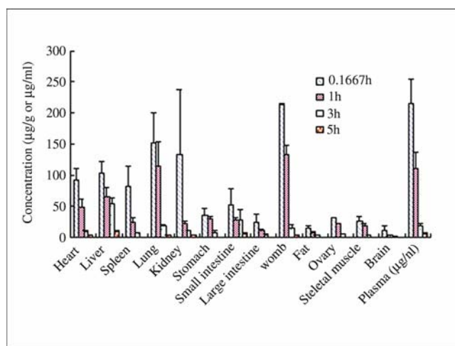
Fig. 3: The concentrations of MPD in the plasma and tissues at 0.1667, 1, 3 and 5 h after an intravenous injection at a dose of 80 mg/kg of MPD to female rats (n = 5)
