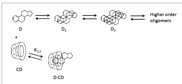
Fig. 3: Formation of drug/cyclodextrin complex in presence of drug dimers ( D_2 ), trimers ( D_3 ) and higher order aggregates that have negligible affinity for the cyclodextrin cavity
