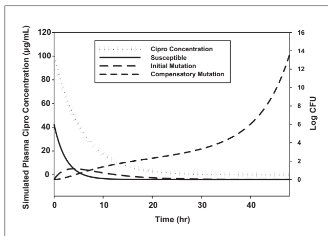
Fig. 3: The time course profiles of PK and subcompartmental PD following single ciprofloxacin treatment in E. coli 204. The dotted line represents the ciprofloxacin concentrations. The solid line represents susceptible bacterial population. The long dashed line describes the minimal mutated population that does not have sufficient bacterial fitness. The short dashed line that accounts for the majority of bacterial re-growth represents the drug resistant population with restored fitness
