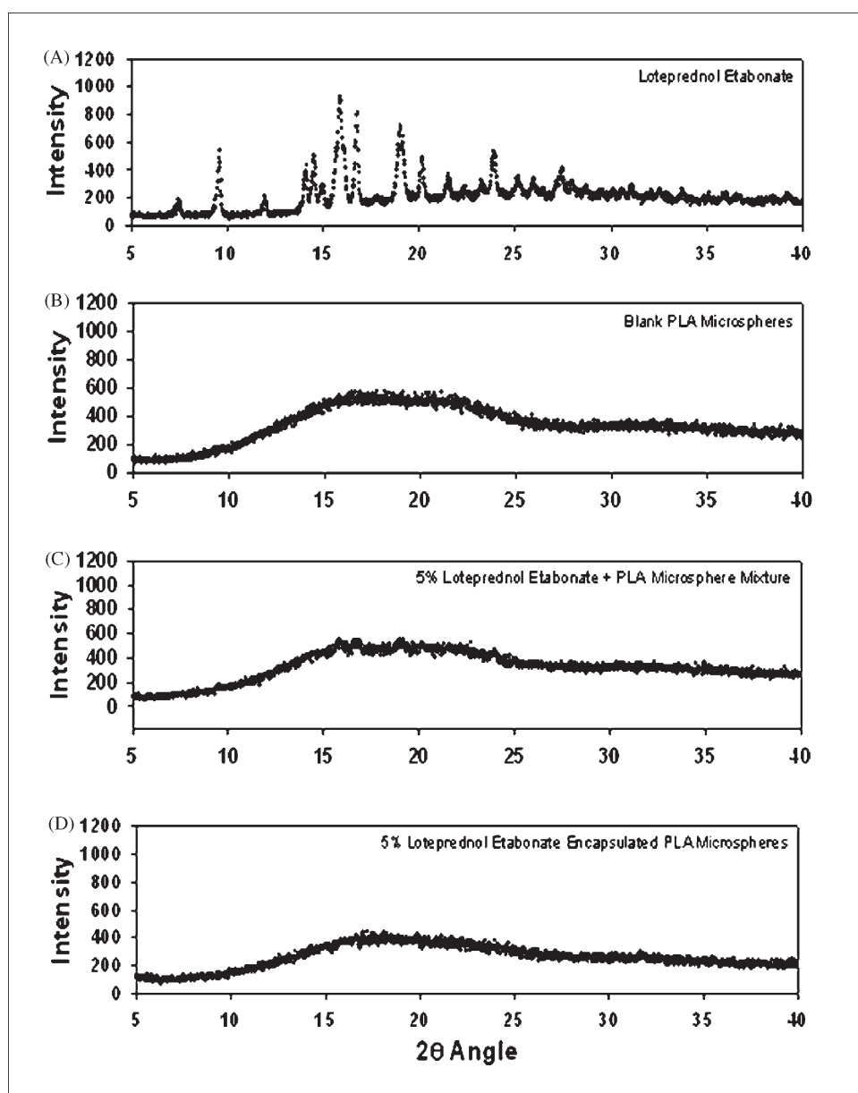
Fig. 4: PXRD patterns of LE (A), blank PLA microspheres (B), their physical mixture (C), and LE-PLA microspheres (D) for particles prepared according to the sonicator method
