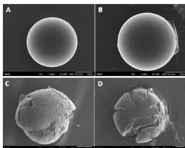
Fig. 5: Scanning electron microscope pictures showing the particle morphology of LE-PLA microspheres during in vitro drug release studies at (A) 0, (B) 4, (C) 8, and (D) 12 months
