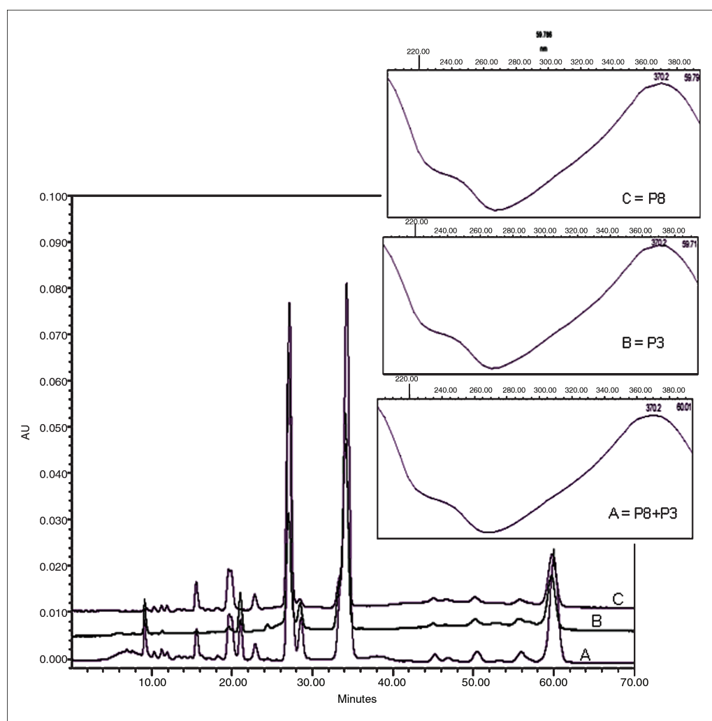
Fig. 6: LC chromatogram of the Achyrocline satureioides spray dried powder SDP40 prepared from ethanol 40 % (v/v) extractive solution plus SDP80 prepared from ethanol 80 % (v/v) extractive solution of the inflorescences (A), SDP40 (B) and SDP80 (C), with respective UV spectra of substances P3 + P8 (SDP40 + SDP80), P3 (SDP40) and P8 (SDP80)
