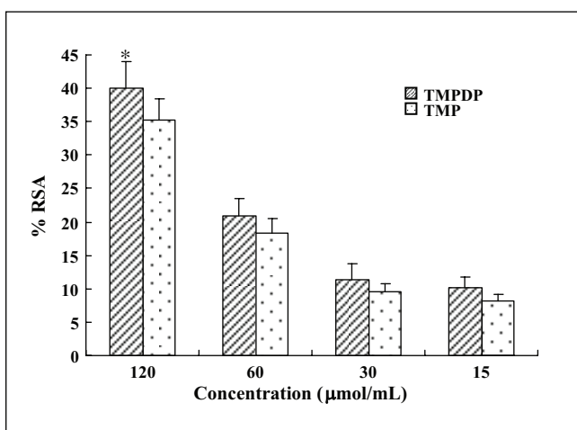
Fig. 2: Effect of TMPDP against DPPH test. For each concentration of TMPDP and TMP tested (15, 30, 60 and 120 \mu\text{mol/ml} ), reduction of DPPH radical was followed by monitoring decrease of absorbance at 516 nm. Data of % RSA expressed as mean \pm S.D. (n = 6). * P < 0.05 , compared with 120 \mu\text{mol/ml} TMP-treated group
