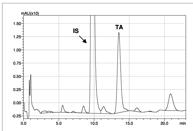
Fig. 2: Representative chromatogram of a stressed solution of triamcinolone acetonide (TA), detection at \lambda = 240 nm
