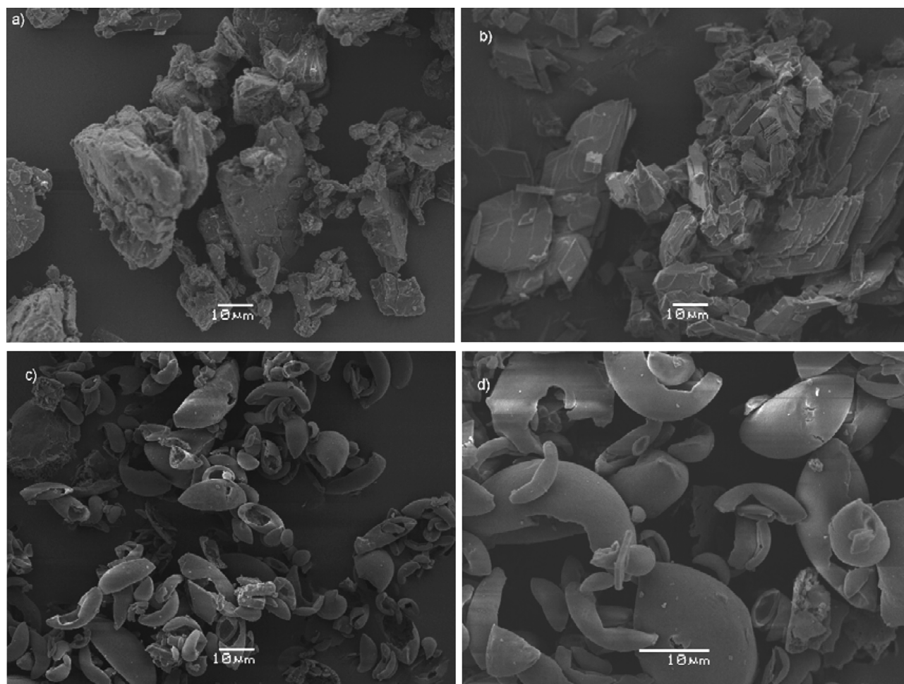
Fig. 2: SEM micrographs of microparticles LVO- \beta CD by precipitation and spray drying techniques: (a) \beta -CD; (b) \beta CD-LVO-PR, and (c) \beta CD-LVO-SD at magnification 1000 times, and (d) \beta CD-LVO-SD at magnification 2000 times
