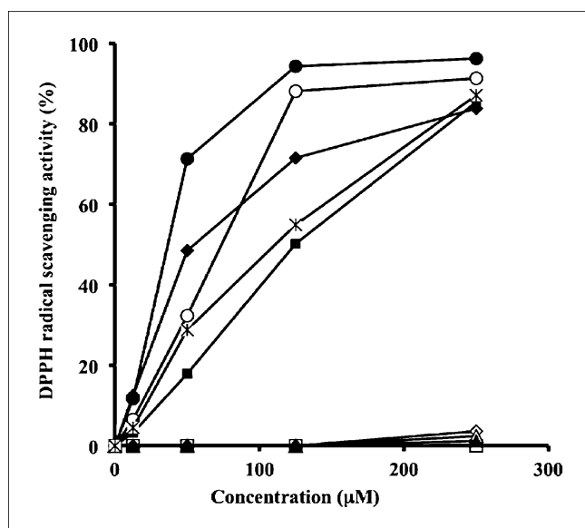
Fig. 2: DPPH radical scavenging activities of dihydro cinnamic acid derivatives (1a-8a). □ Dihydro cinnamic acid (1a), ◇ Dihydro- p -coumaric acid (2a), △ Dihydro- p -methoxy cinnamic acid (3a) ◇ Dihydro caffeic acid (4a), ■ Dihydro ferulic acid (5a), ◆ Dihydro isoferulic acid (6a), ▲ 3,4-Dimethoxy-dihydro cinnamic acid (7a), ◆ Dihydro sinapic acid (8a), ✕ BHT
