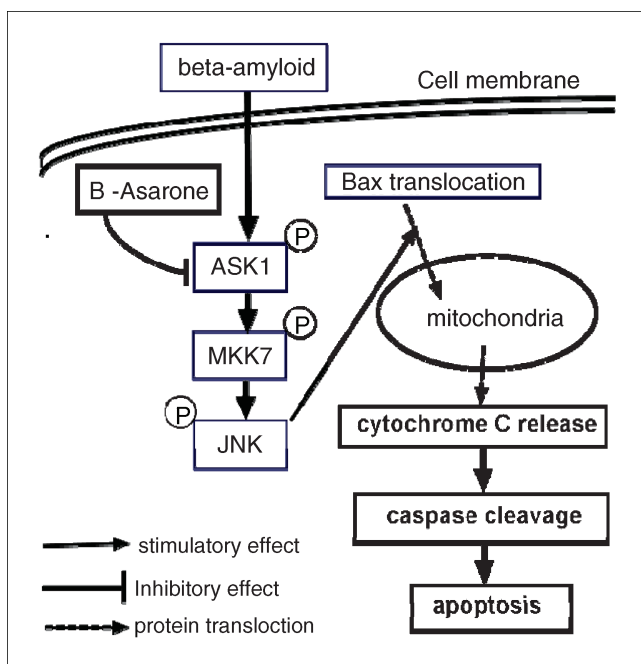
Fig. 4: Schematic representation of molecular mechanisms of \beta -Asarone inhibits the apoptosis in SH-SY5Y cells induced by \beta A. \beta A induces ASK1 phosphorylation. ASK1 phosphorylation, in turn, increases MKK7 phosphorylation, which serve to increase JNK phosphorylation. JNK activation induces the mitochondrial pathway of apoptosis involving increased expression of Bax and Bad, followed by mitochondrial release of cytochrome c . Release of cytochrome c then further induces caspase-9 activation, leading caspase-3 activation and apoptosis. \beta -Asarone reverse above-mentioned incident
