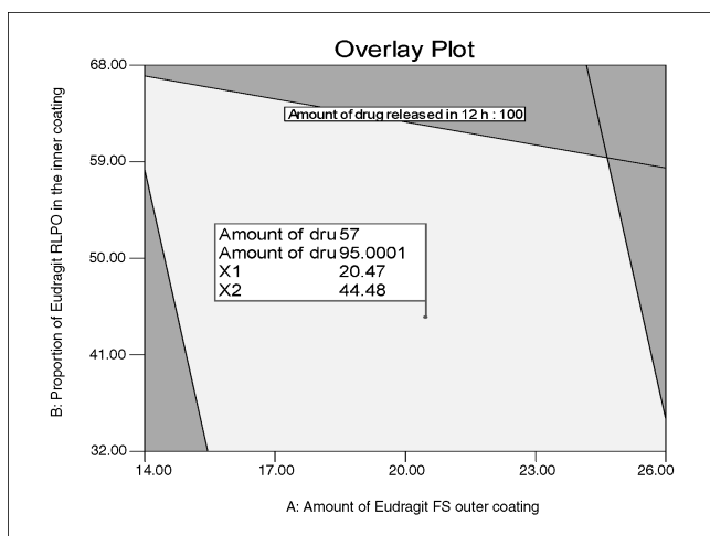
Fig. 7: Overlay plot for optimization
