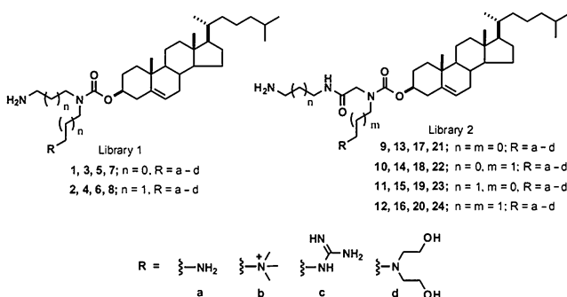
Fig. 6: Structures of new asymmetrical polar head cholesterol-based cationic lipids (Radchatawedchakoon et al. 2010)
