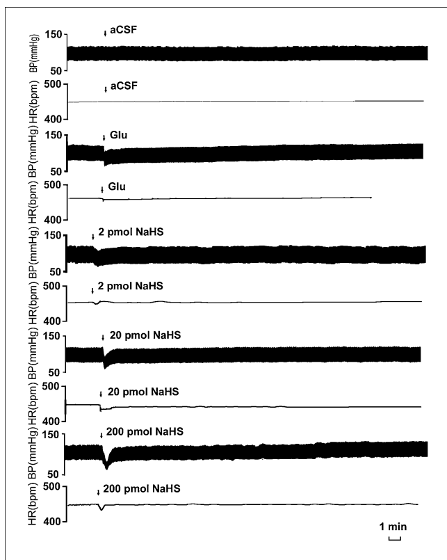
Fig. 1: TOP: Representative tracings showing BP and HR responses to unilateral microinjection of aCSF, Glu or NaHS (2, 20, 200 pmol) into the NTS in anaesthetized and paralyzed rats (A). BUTTON: The functional region of the NTS was identified by the depressor effects of L-Glu (5 nmol)
