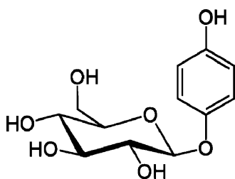
Fig. 1: The chemical structure of arbutin.
