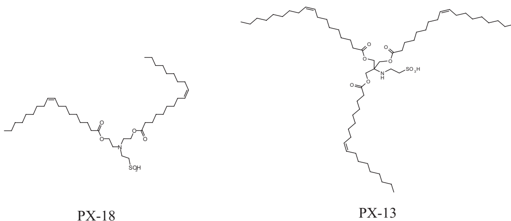
Fig. 1: Chemical structure of the sPLA 2 -IIA inhibitors PX-18 and PX-13
