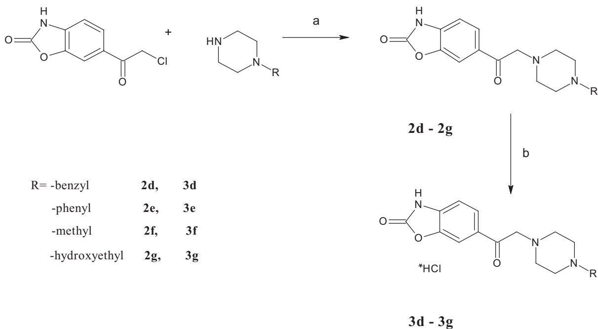
Scheme 2: Scheme of synthesis of 6-chloroacetyl-2-benzoxazolinone with N-substituted piperazine derivatives (a) acetone/60 °C/2-4 h/reflux; (b) HCl/methanol
