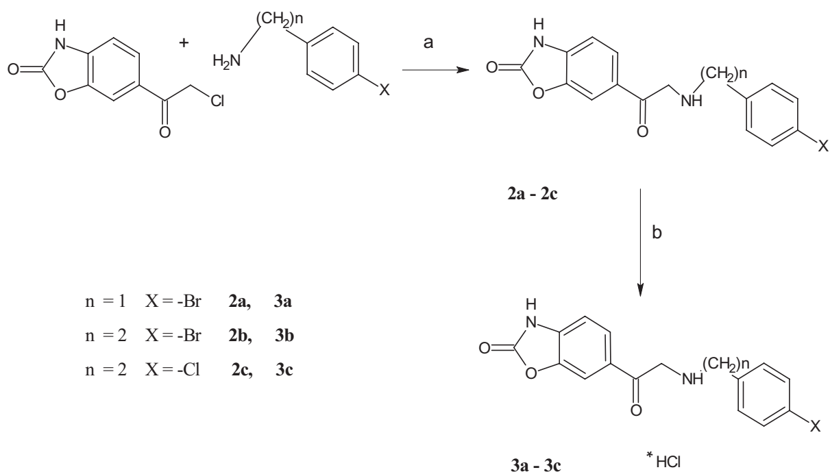
Scheme 1: Scheme of synthesis of 6-chloroacetyl-2-benzoxazolinone with 4-substituted aryl-aliphatic amine derivatives (a) acetonitrile/80 °C/2 h/reflux; (b) HCl/methanol
