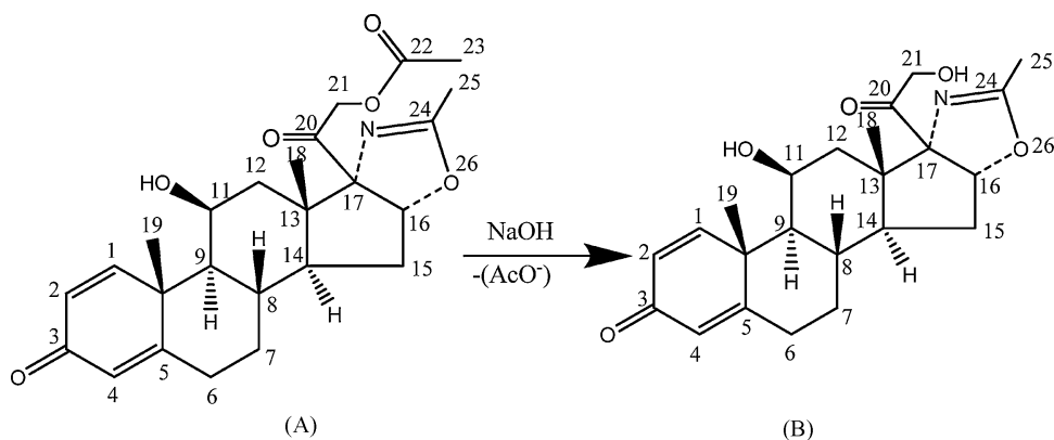
Scheme: Chemical structure of DFZ (DFZ) (A) and its degradation product- DDP1: 21-hydroxy deflazacort (B)
