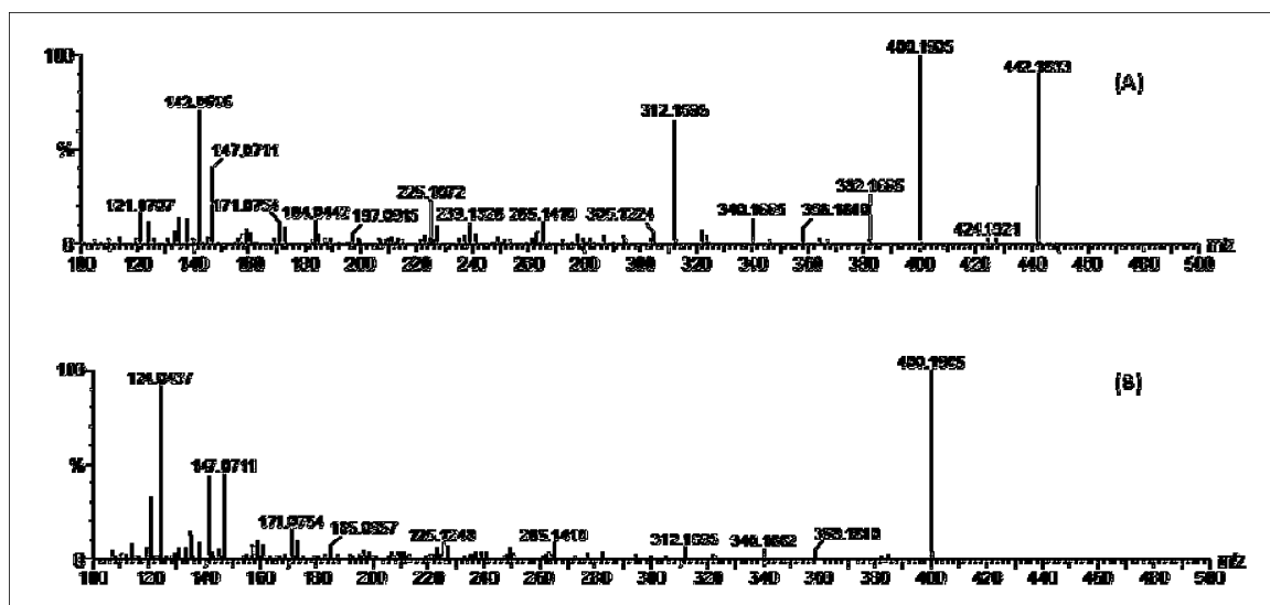
Fig. 2: LC-MS of DFZ (A) and DDP1 (B)
