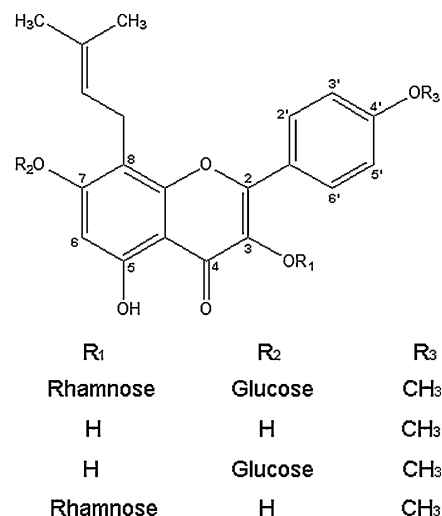
Fig. 2: Chemical structures of icariin and its metabolites.
