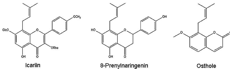
Fig. 3: Structures of icariin, 8-prenylnaringenin and osthole.
