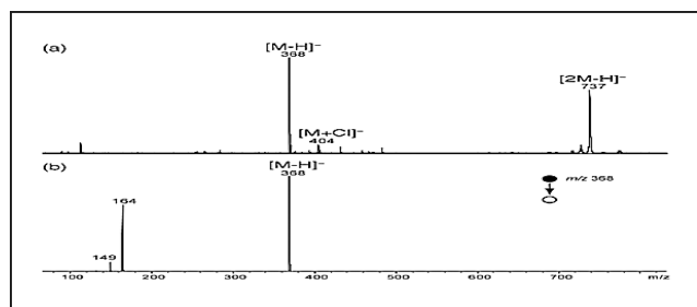
Fig. 4: (a) ESI spectrum of lansoprazole recorded in the negative ion mode and (b) CID spectrum of the [M-H]^- ion m/z 368.
