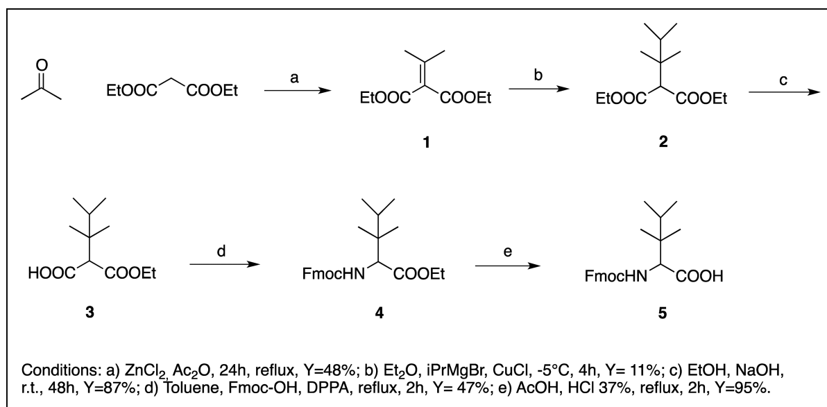
Scheme: Synthetic approach adopted for the synthesis of racemic 2-amino-3,3,4-trimethyl-pentanoic acid.
