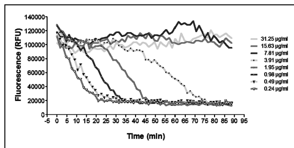
Fig. 2: Representative example of radical scavenging activity of nilocitin [2,3-Di- O -galloyl-( \alpha/\beta )-glucopyranose ( 2 )] measured by ORAC assay. Concentration tested ranged from 31.25 to 0.24 \mu\text{g}/\text{ml} . Relative fluorescence was constant over the whole measurement period up to a concentration of 7.81 \mu\text{g}/\text{ml} demonstrating high antioxidant activity with an \text{ED}_{50} of 4.95 \mu\text{g}/\text{ml} .
