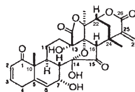
Physalin A
