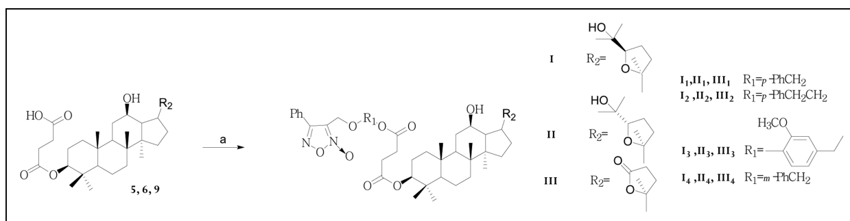
Scheme 3: Synthesis of final products (compounds I 1-4 , II 1-4 , III 1-4 ) Reagents and conditions: a) A 1-4 , DMAP, EDCI, 25^\circ\text{C} , \text{CH}_2\text{Cl}_2 , 6 h.
