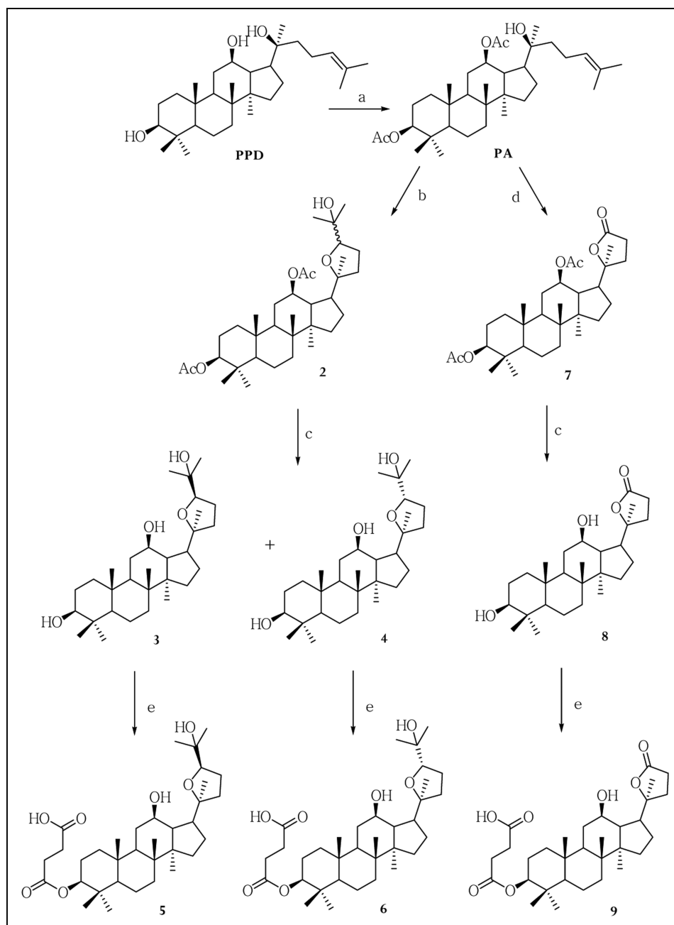
Scheme 2: Synthesis of the derivatives from PPD (compounds 5 , 6 , 9 ) Reagents and conditions: a) (\text{CH}_3\text{CO})_2\text{O} , DMAP, \text{CHCl}_3 , r.t., 12 h; b) m -CPBA, \text{CH}_2\text{Cl}_2 , -3^\circ\text{C} , 5 h; c) \text{NaOH} , \text{H}_2\text{O} , \text{CH}_3\text{OH} , reflux, 6 h; d) \text{CrO}_3 , \text{CH}_3\text{COOH} , \text{H}_2\text{O} , r.t., 3 h; e) Succinic anhydride, DMAP, \text{CHCl}_3 , 42^\circ\text{C} , 6 h.
