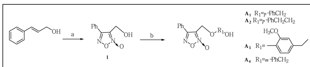
Scheme 1: Synthesis of furoxans A 1-4 Reagents and conditions: a) NaNO 2 , HOAc, r.t., 1 h; b) (i) SOCl 2 , pyridine, CH 2 Cl 2 , r.t., 8 h; (ii) HOR 1 OH, K 2 CO 3 , KI, CH 3 CN, r.t., 3 h.
