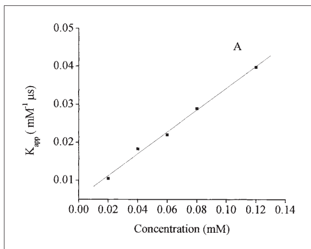
Fig. 6: Dependence of first-order rate constant for the growth of absorbance at 480 nm on [quercetin] on pulse irradiation of 0.2 M \text{Na}_2\text{CO}_3 aqueous solution containing quercetin saturated with \text{N}_2\text{O}
