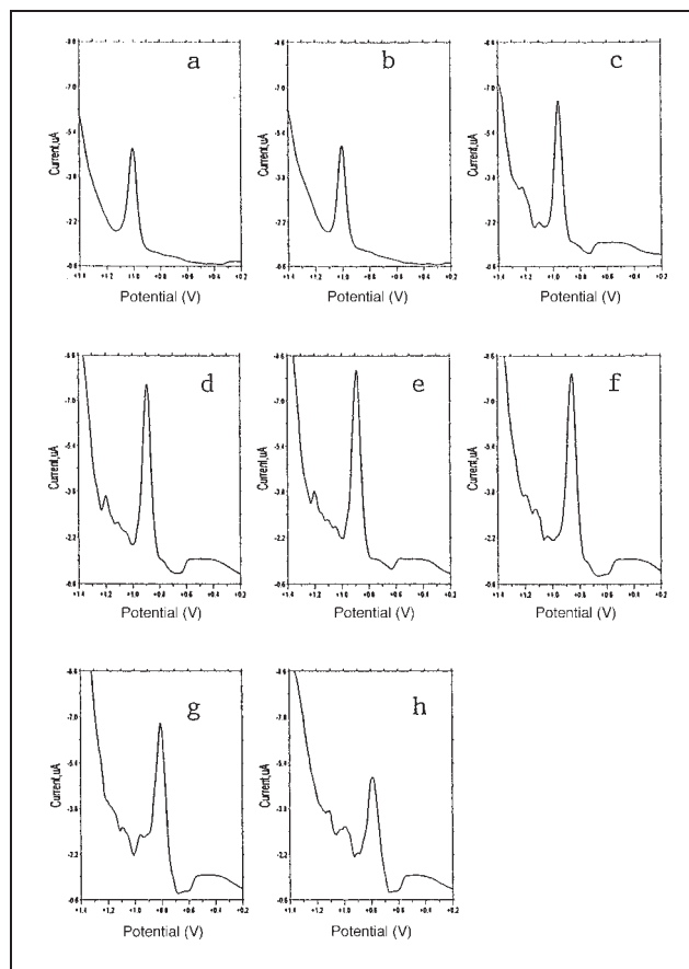
Fig. 4: Differential pulse voltammograms recorded in BR buffers of different pH containing 1.0 \times 10^{-4} \text{ M} DOR, scan rate 20 \text{ mVs}^{-1} . a) \text{pH} = 1.53 ; b) \text{pH} = 2.02 ; c) \text{pH} = 2.87 ; d) \text{pH} = 3.06 ; e) \text{pH} = 5.00 ; f) \text{pH} = 6.01 ; g) \text{pH} = 7.24 ; h) \text{pH} = 8.16 . Scan rate 20 \text{ mV} \cdot \text{s}^{-1} , pulse amplitude 50 \text{ mV} ; sample width 17 \text{ ms} , pulse width: 50 \text{ ms} , pulse period 200 \text{ ms} .
