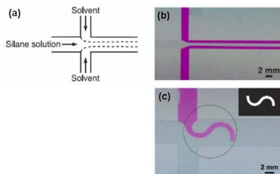
Figure 1. (a) Schematic illustration of multistream laminar flow and the corresponding images of aqueous flow inside channel after surface patterning (b). The liquid is a dilute solution of Rhodamine B dye (0.057 w/w %) in deionized water. (c) A dilute Rhodamine B aqueous solution was added into the channels by a syringe, and a pressure was applied to push the solution slowly through the hydrophobic region. When the aqueous solution reached the edge of the irradiated area, it wetted the hydrophilic region spontaneously and formed patterns identical to the photomasks, shown at a reduced size in the upper right corner. “Reproduced with permission of 28”.
